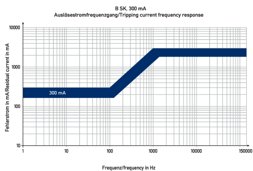
Diagramme FI-/LS-Kombinationen DRCBO 4 Co6/0,30/1N-B SK
