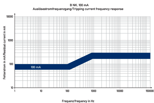
Diagramme FI-/LS-Kombinationen DRCBO 4 B16/o,10/3N-B NK
