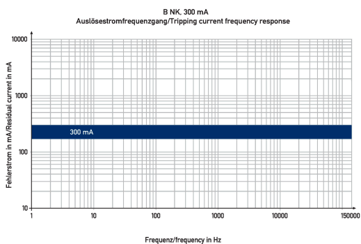
Diagramme FI-/LS-Kombinationen DRCBO 4 B16/o,30/1N-B NK
