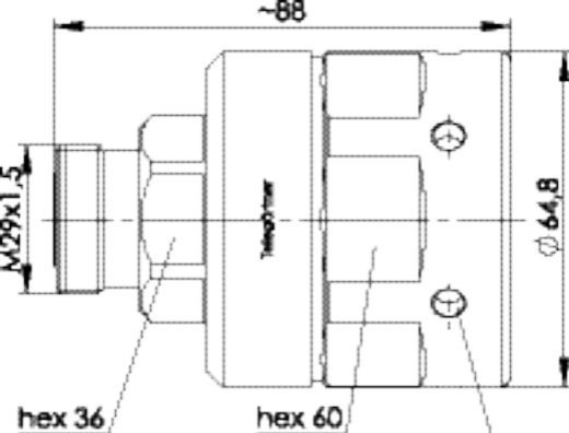
hook wrench DIN 1818-B 68-75 Hakenschlüssel
