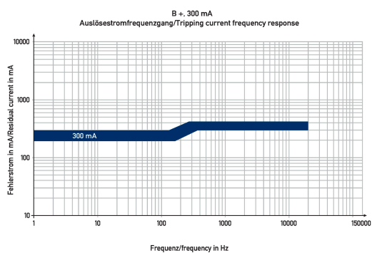
Diagramme FI-/LS-Kombinationen DRCBO 4 Co6/0,30/3N-B+
